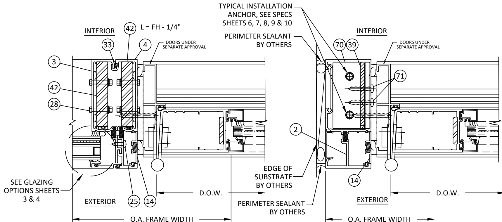
R 16 HORIZONTAL SECTION JAMB - CONCRETE/MASONRY W/ 1X BUCK STANDARD CONFIGURATION
