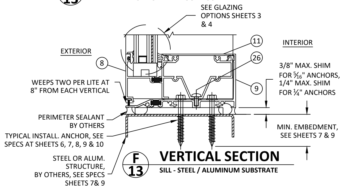
E 13 VERTICAL SECTION HEAD WITH RECEPTOR - 2X WOOD BUCK
