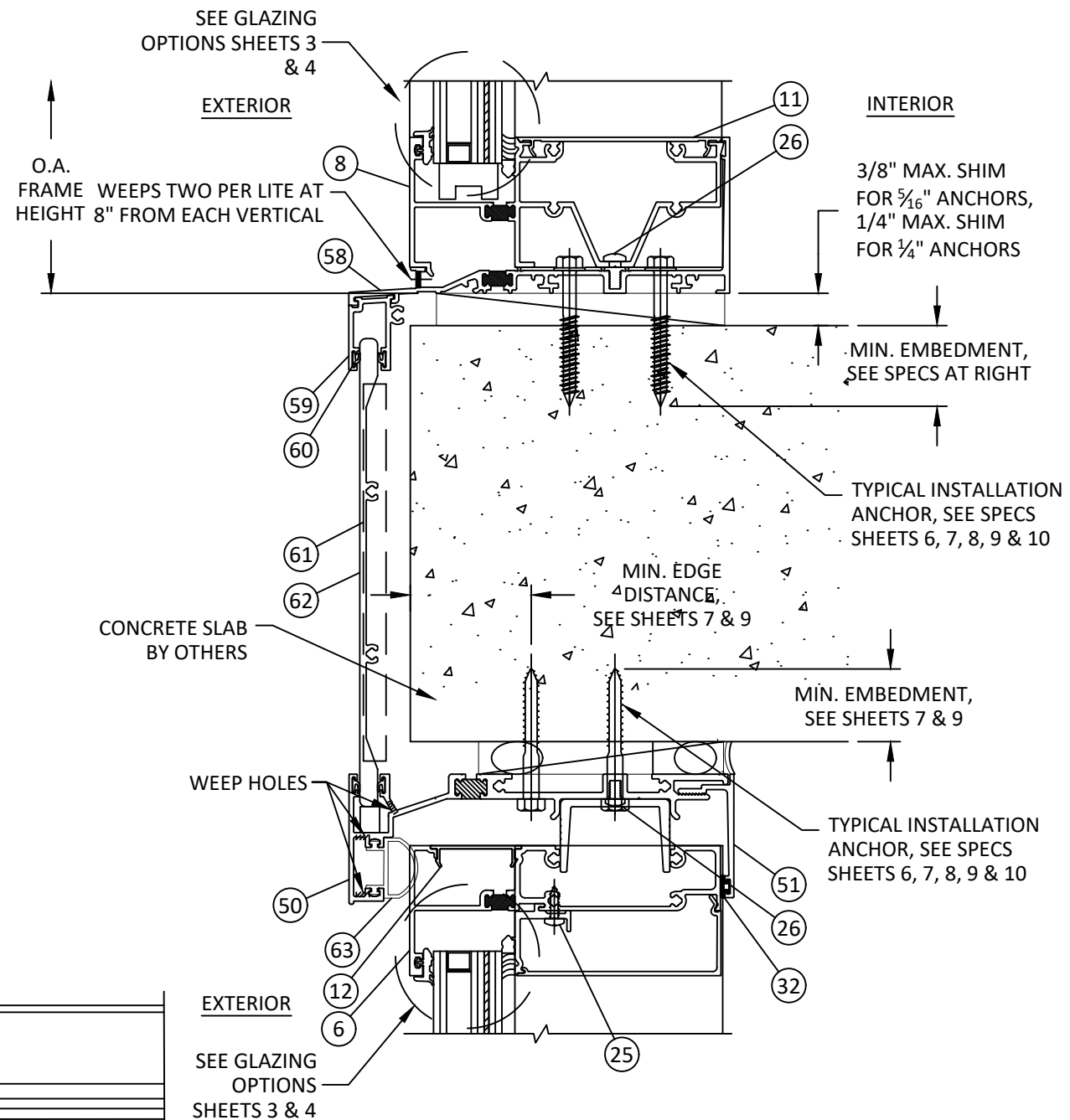
T 16 HORIZONTAL SECTION SLAB EDGE CONFIGURATION
