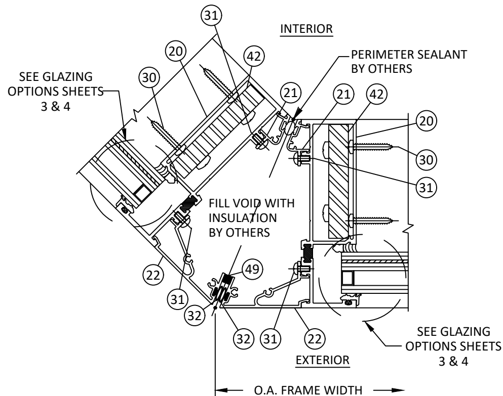
M 15 HORIZONTAL SECTION 135° OUTSIDE CORNER STANDARD CONFIGURATION
