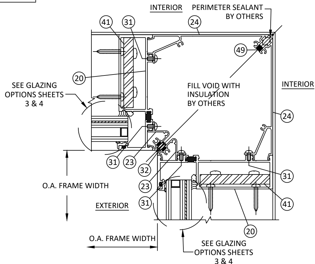
P 15 HORIZONTAL SECTION 90° INSIDE CORNER STANDARD CONFIGURATION
