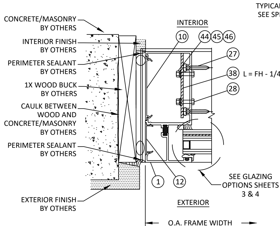
G HORIZONTAL SECTION 14 JAMB - CONCRETE/MASONRY W/ 1X BUCK STANDARD CONFIGURATION
