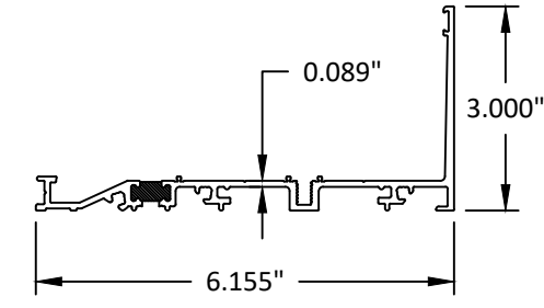
9 SILL FLASHING
