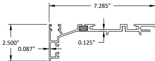
50 HEAD RECEPTOR
