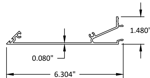
24 90° CORNER COVER (LARGE)
