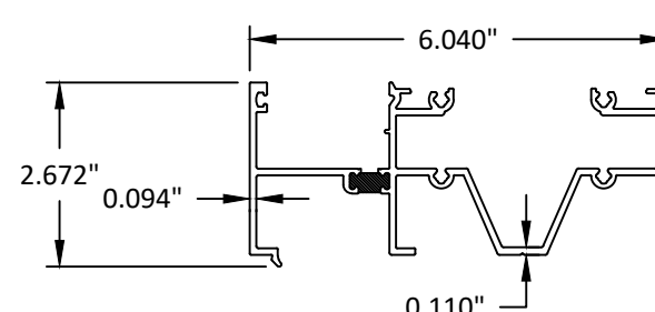
8 SILL
