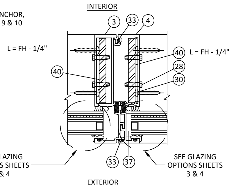
I HORIZONTAL SECTION 14 MULLION - CONCRETE/MASONRY W/ 1X BUCK STANDARD CONFIGURATION
