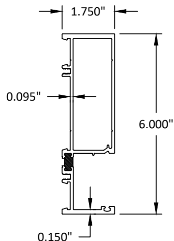
20 CORNER MULLION HALF
