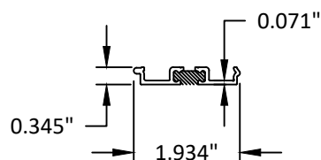
14 FLAT FILLER
