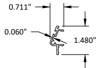
21 135° CORNER COVER (SMALL)
