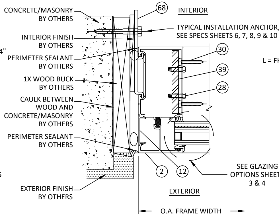
H HORIZONTAL SECTION 14 JAMB - CONCRETE/MASONRY W/ 1X BUCK STANDARD CONFIGURATION
