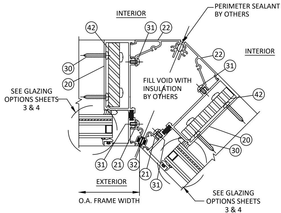
O 15 HORIZONTAL SECTION 135° INSIDE CORNER STANDARD CONFIGURATION
