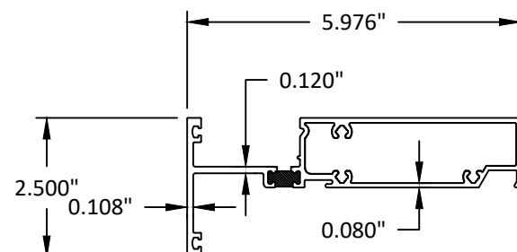
7 HORIZONTAL
