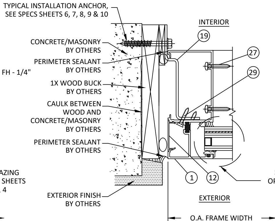
H HORIZONTAL SECTION 14 JAMB - CONCRETE/MASONRY W/ 1X BUCK STANDARD CONFIGURATION
