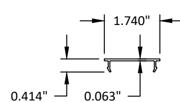
12 PVC PERIMETER FILLER
