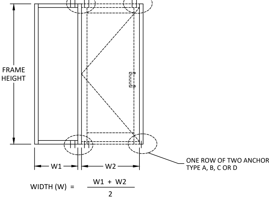
SINGLE DOOR
