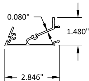
22 135° CORNER COVER (LARGE)
