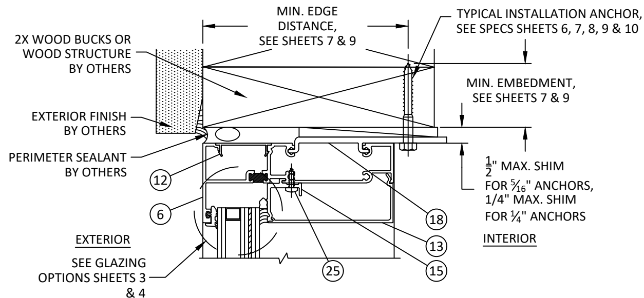
D 13 VERTICAL SECTION HEAD - 2X WOOD BUCK
