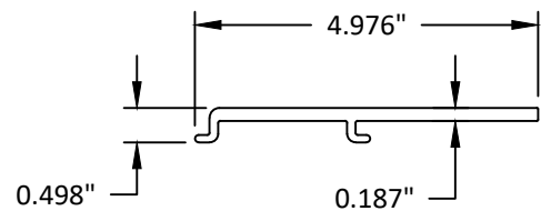
18 STRAP ANCHOR
