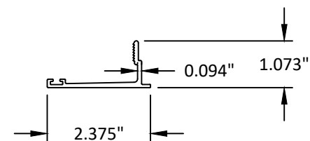
51 RECEPTOR SNAP COVER
