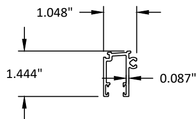
59 ALUMINUM PLATE ADAPTOR
