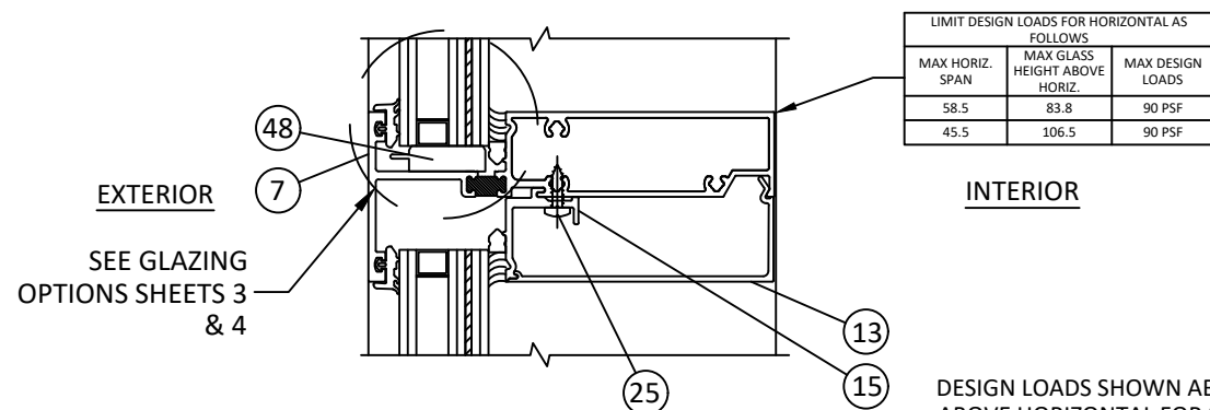
B 13 VERTICAL SECTION HORIZONTAL
