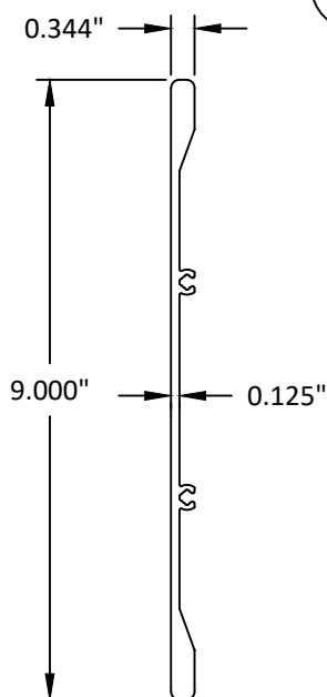
62 9" SLAB EDGE COVER
