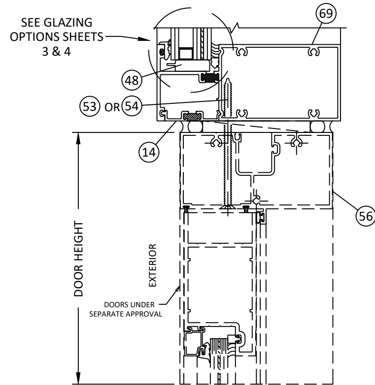
Q 16 VERTICAL SECTION JAMB - CONCRETE/MASONRY W/ 1X BUCK STANDARD CONFIGURATION
