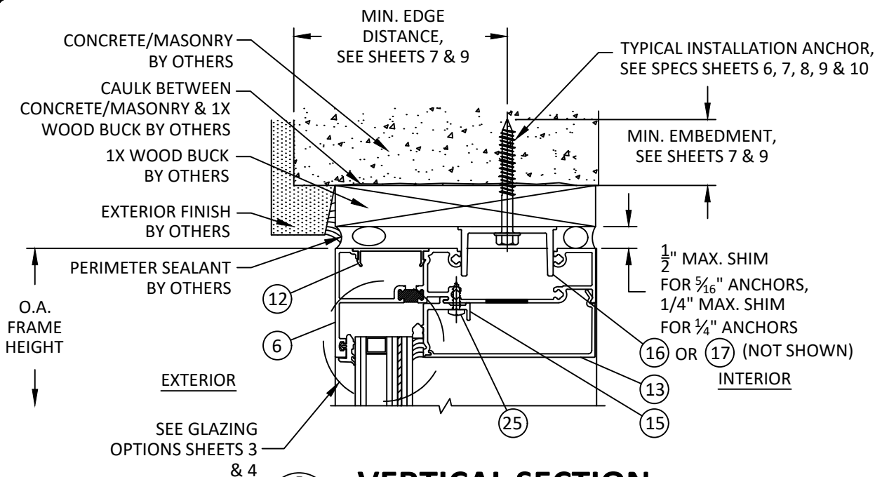
A 13 VERTICAL SECTION HEAD - CONCRETE/MASONRY W/ 1X BUCK
