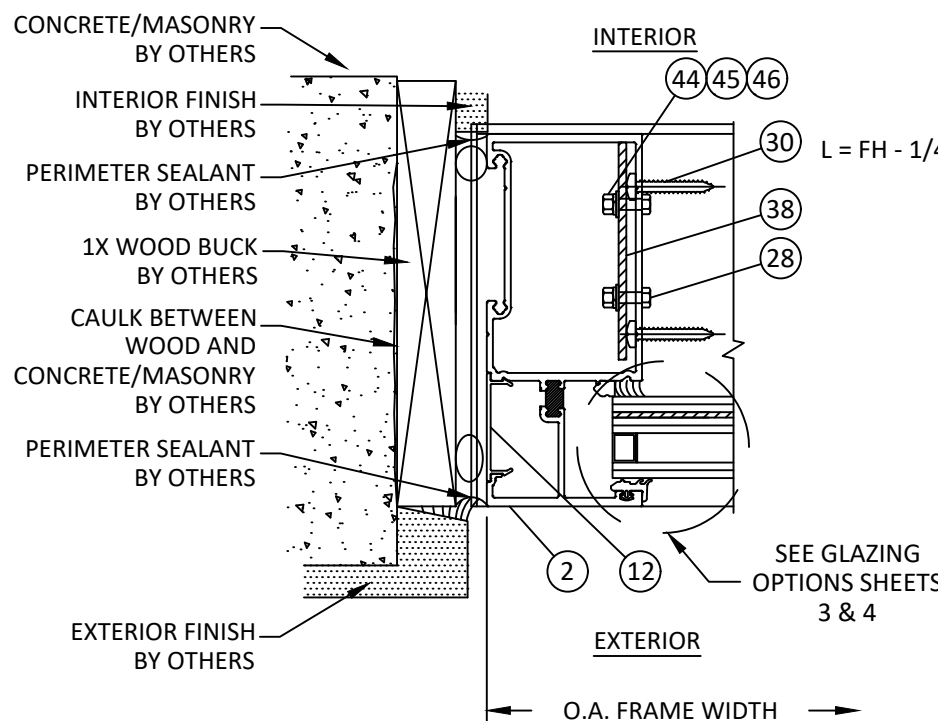
J HORIZONTAL SECTION 14 JAMB - CONCRETE/MASONRY W/ 1X BUCK STANDARD CONFIGURATION
