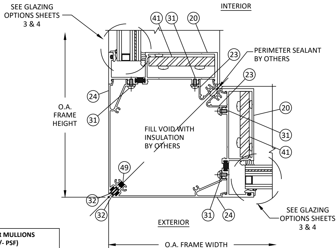
N 15 HORIZONTAL SECTION 90° OUTSIDE CORNER STANDARD CONFIGURATION
