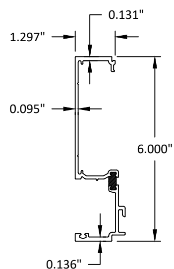
3 MALE MULLION
