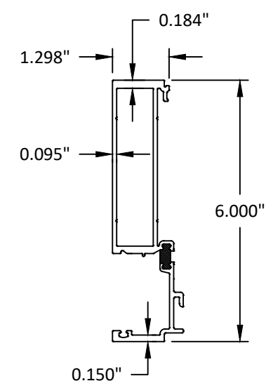
5 HEAVY DUTY MALE MULLION
